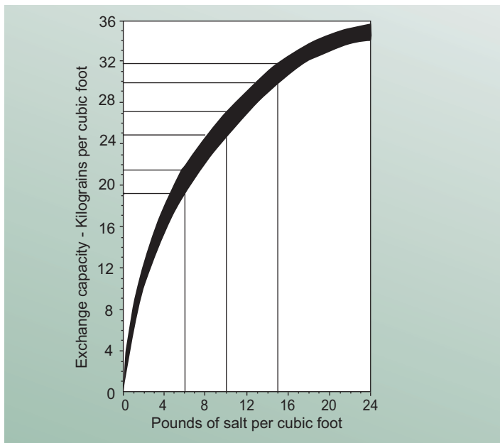
Fig. 1 Exchange capacity vs. regeneration level Sodium form C-800x10 LT Cation Resin
